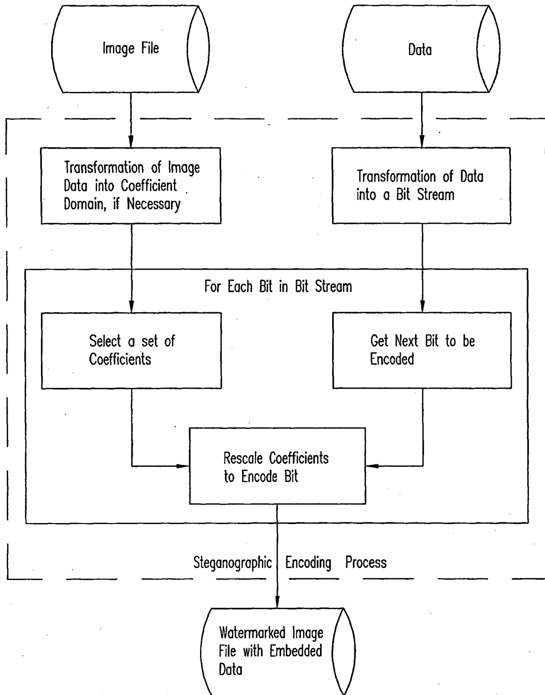
Encoding Data in an Image File
